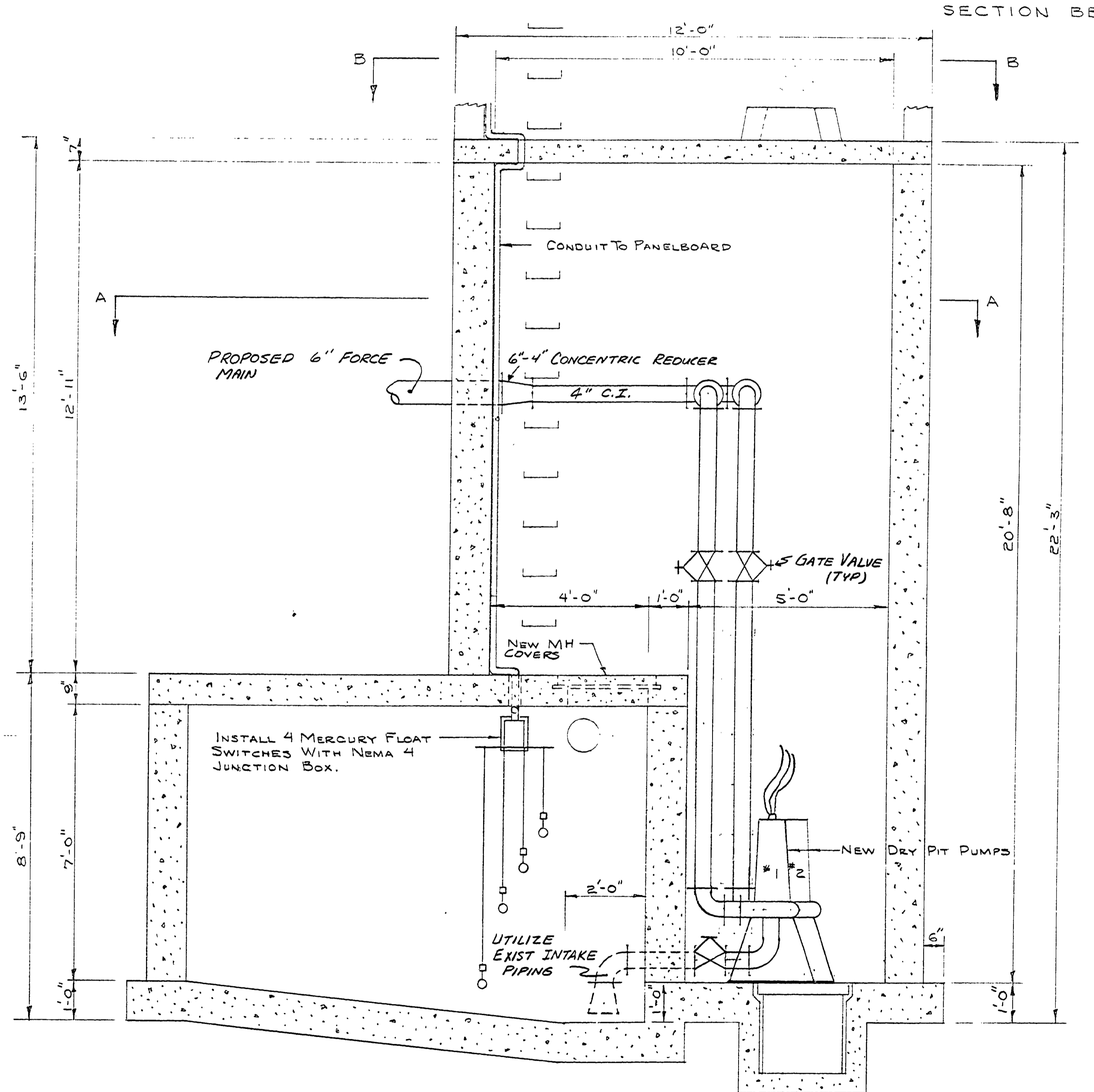
SECTION C-C SCALE 1/2" = 1'-0"
